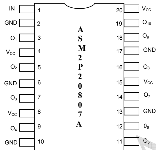
SSOP/ QSOP PACKAGE TOP VIEW
