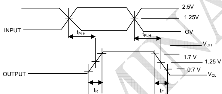
Propagation Delay
