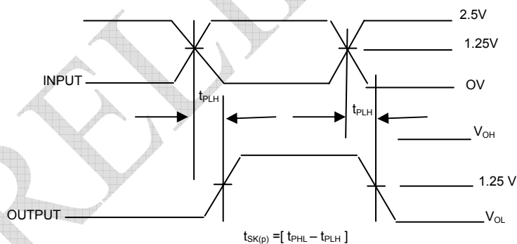
Pulse Skew - t_{SK(P)}
