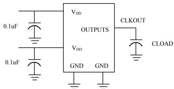
TEST CIRCUIT # 1
