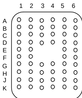
56-BALL BGA (SEE TABLE BELOW)
