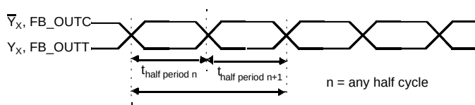
Figure 8: Half-Period Jitter
