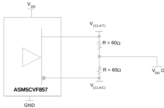
Figure 1: IBIS Model Output Load
