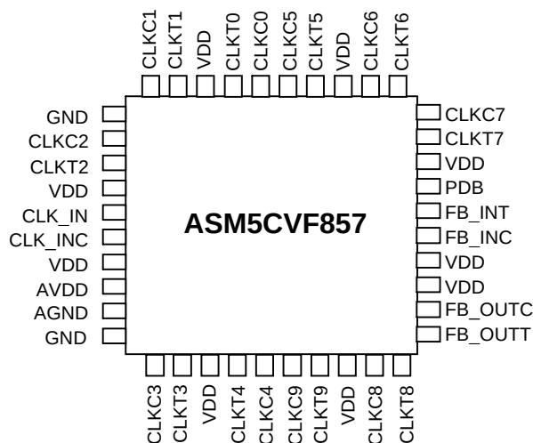
40-PIN MLF
