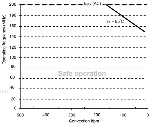
Figure 9. Maximum ASM5I961P frequency, V_{CC} = 3.3V , MTBF 9.1 years, driving series terminated transmission lines
