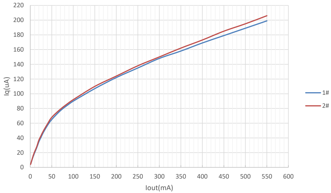
I_q VS. I_{out} ( V_{in}=13.5V )
