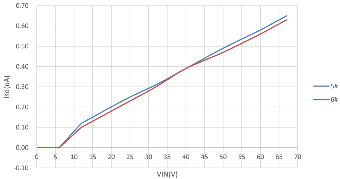
I_{sd} VS. V_{IN} (ON/OFF=5V, I_{out}=0 )
