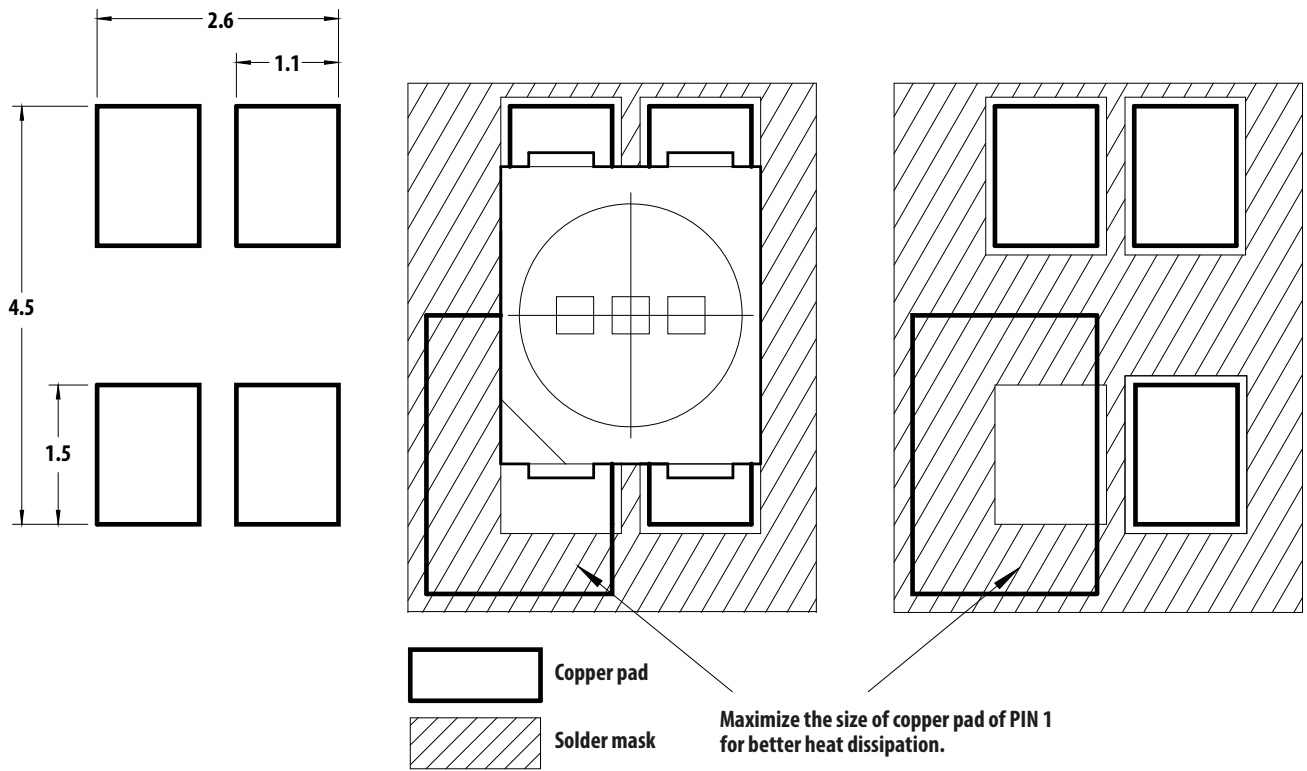
Figure 12. Recommended soldering land pattern
