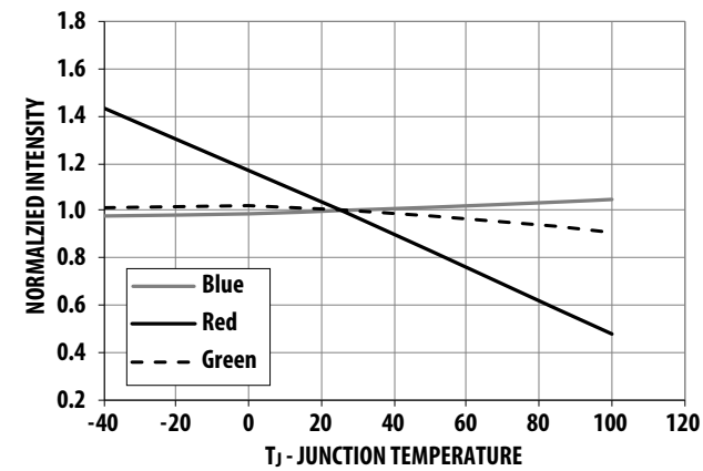
Figure 5. Relative Intensity vs Junction Temperature
