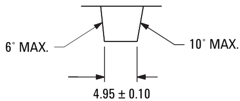
Figure 10. Tape Dimensions
