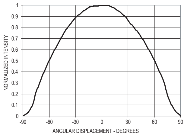
Figure 6. Radiation pattern.
