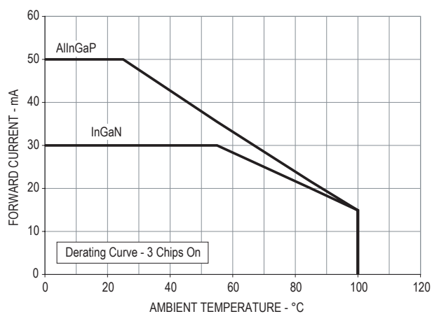
Figure 5a. Maximum forward current vs. ambient temperature. Derated based on T_{JMAX} = 125^{\circ}\text{C} , R\Theta_{JA} = 600^{\circ}\text{C/W} (3 chip on).
