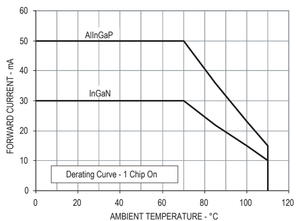
Figure 5b. Maximum forward current vs. ambient temperature. Derated based on T_{JMAX} = 125^{\circ}\text{C} , R\Theta_{JA} = 340^{\circ}\text{C/W} (1 chip on).
