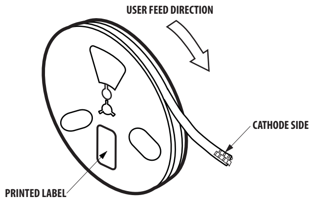
Figure 14. Reeling Orientation
