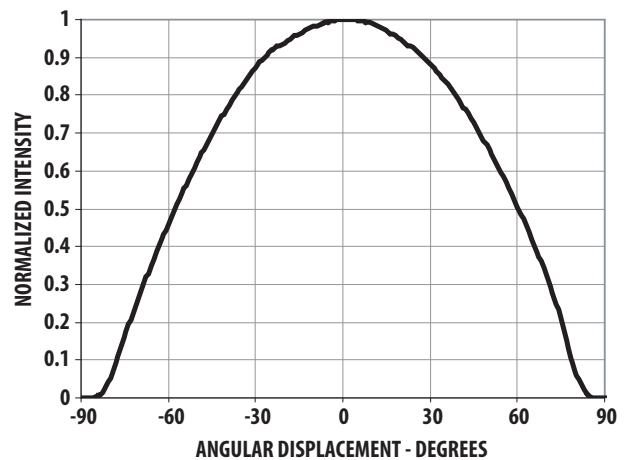
Figure 8. Radiation Pattern
