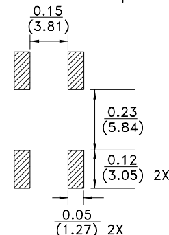
Dimensions: Inches (mm)
