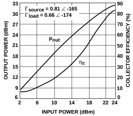
Figure 7. Output Power and Collector Efficiency vs. Input Power.
