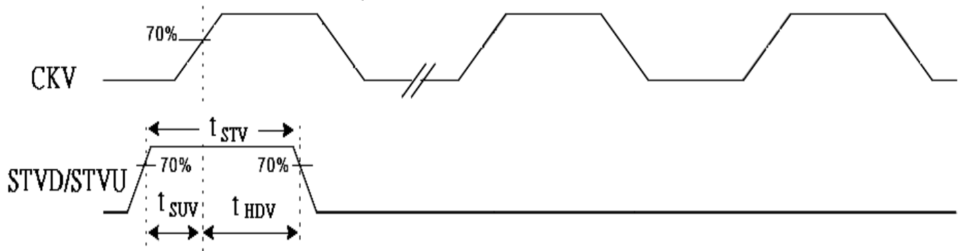
Fig.3-6 STV Start pulse timing
