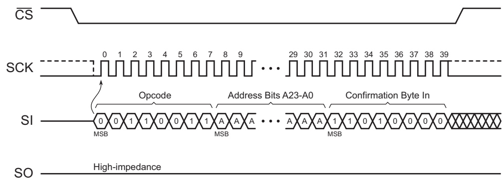
Figure 10-1. Sector Lockdown
