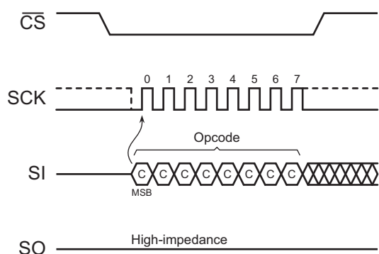
Figure 8-8. Chip Erase
