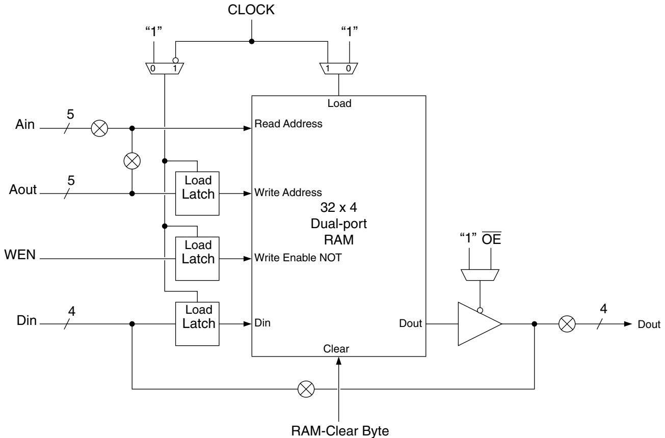
Figure 8. RAM Logic
