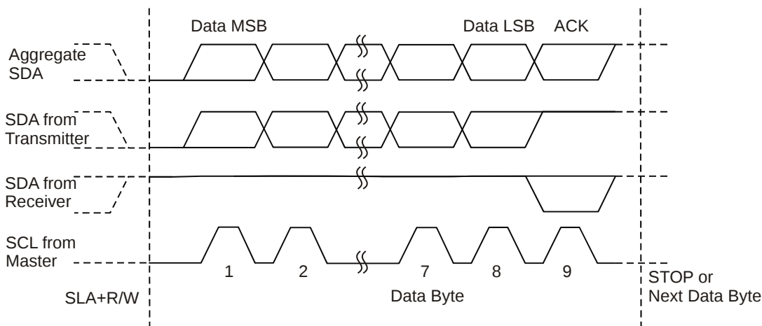
Figure 4-7. Packet Transmission
