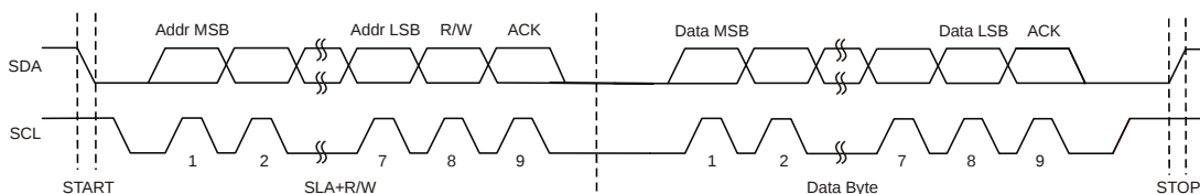
Figure 4-7. Packet Transmission
