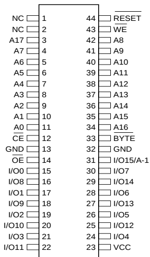
AT49F4096A(T) SOIC (SOP)
