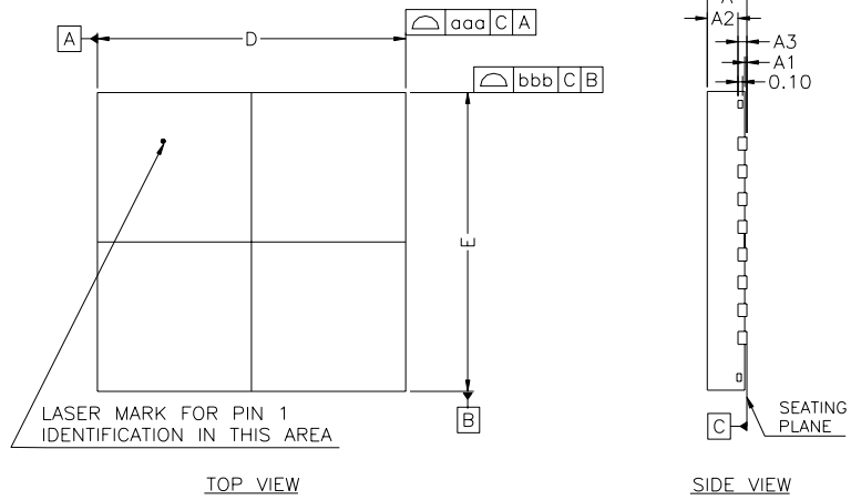
Figure 13-1. Package Outline
