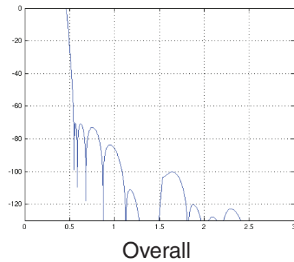
Figure 12-17. ADC Type 1 Frequency Response
