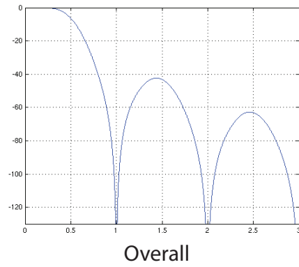
Figure 12-15. DAC Type 4 Frequency Response
