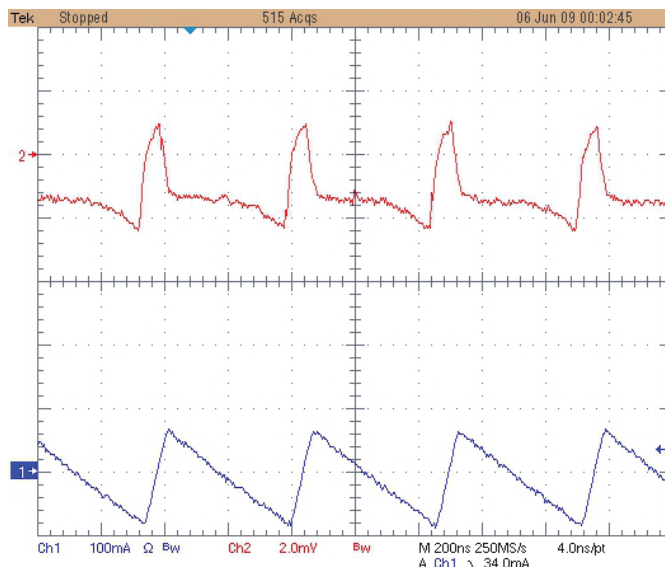
DCDC1 - V IN = 5.5V - V OUT = 1.2V Output Voltage Ripple
