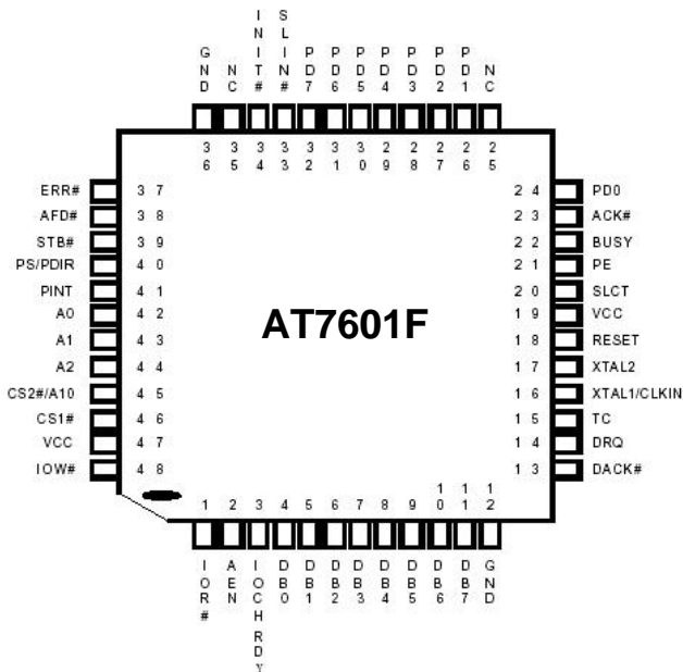
Figure 1. AT7601F Pin Diagram (Top View)
