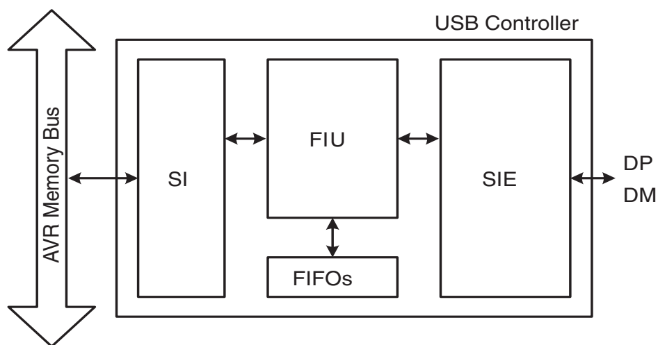
Figure 6-7. USB Controller
