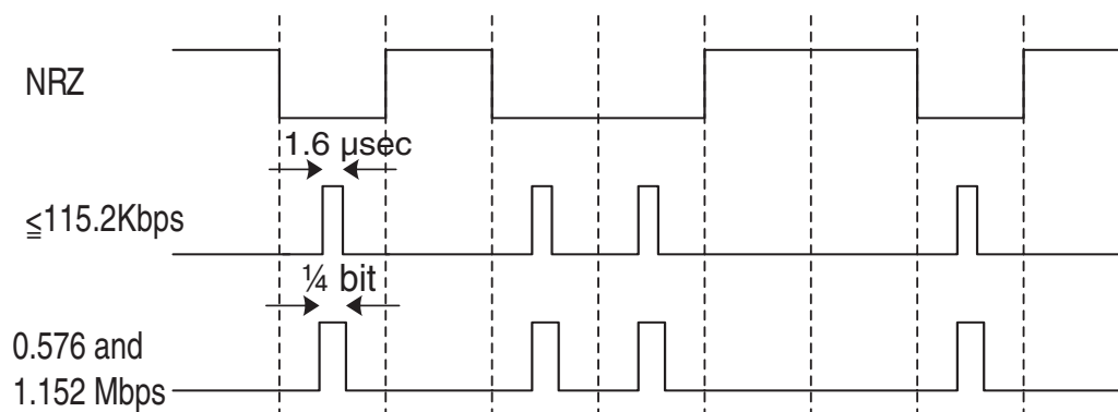
Figure 6-10. Pulse Duration
