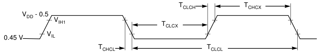
Figure 24-29. AC Testing Input/Output Waveforms
