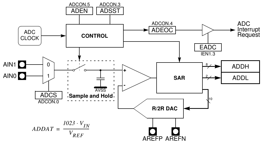
Figure 22-1. ADC Structure
