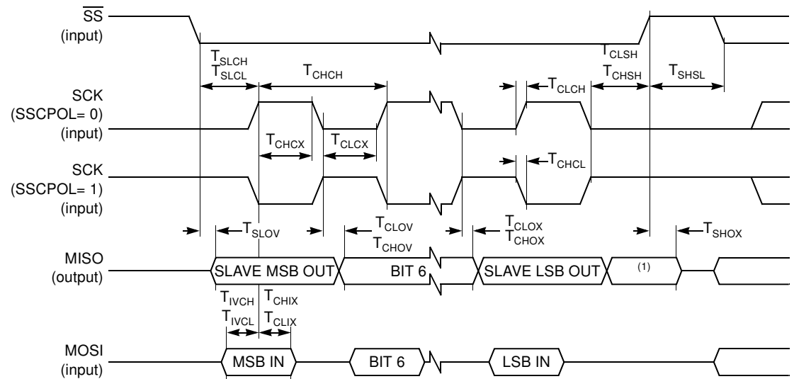
Figure 24-19. SPI Slave Waveforms (SSCPHA= 0)
