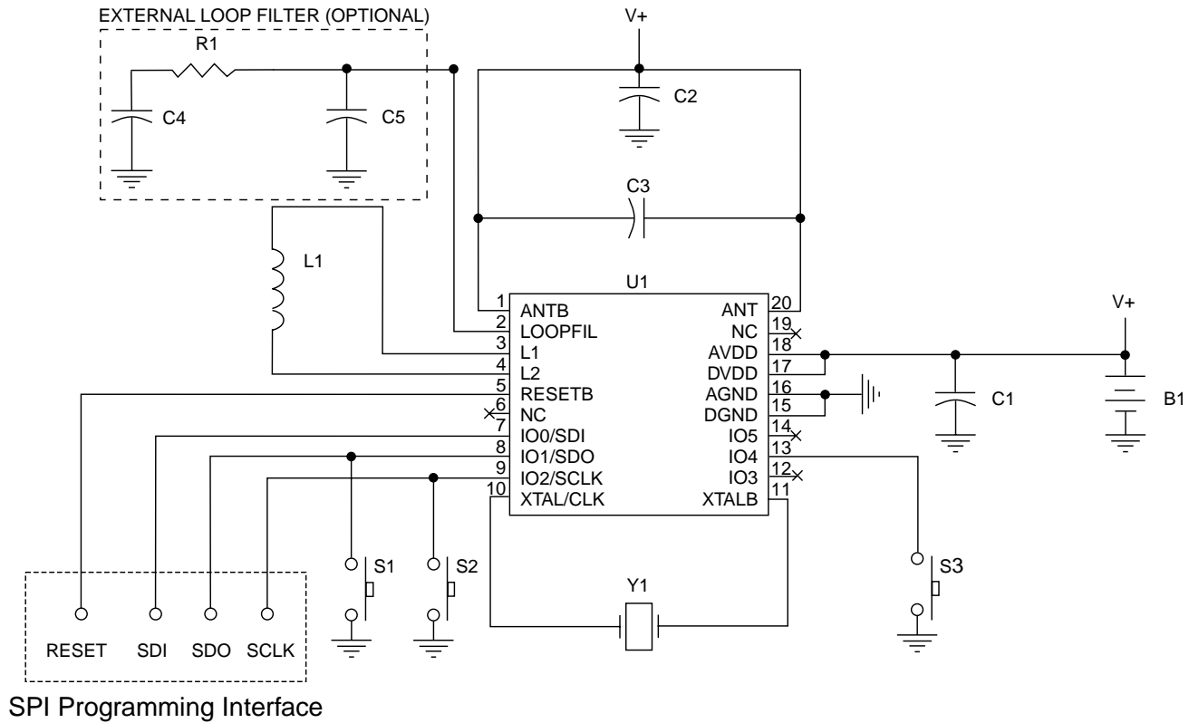
Figure 3. Sample Circuit
