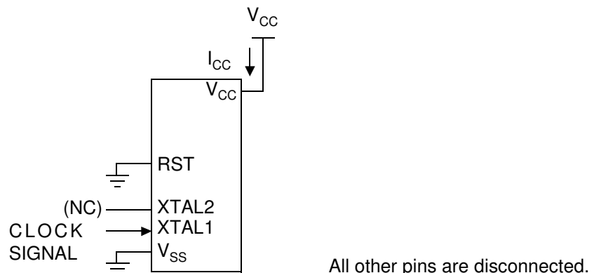
Figure 38. I_{CC} Test Condition, under reset
