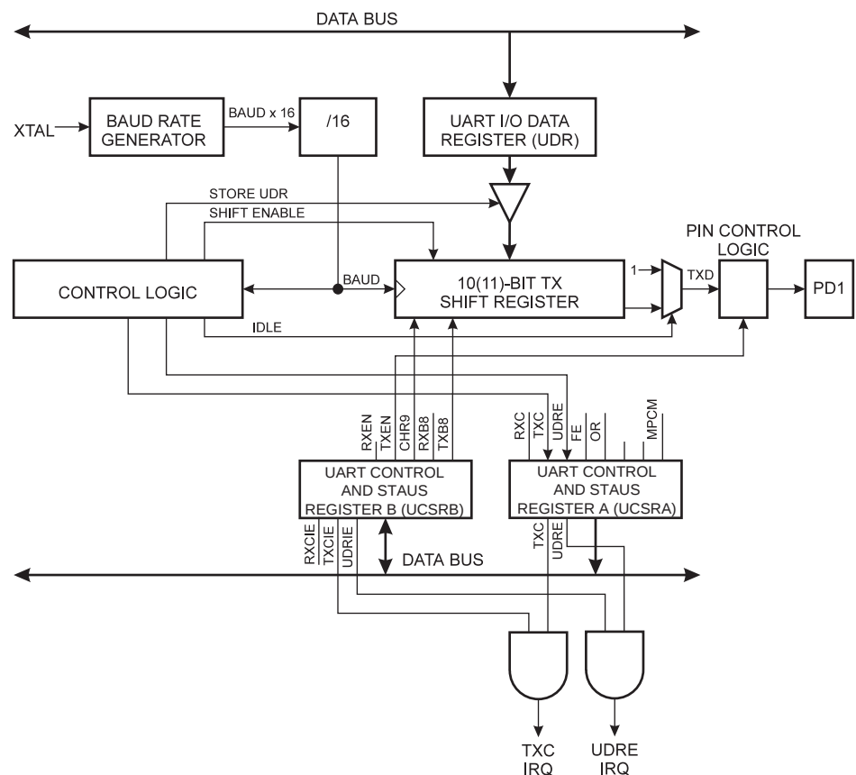
Figure 40. UART Transmitter
