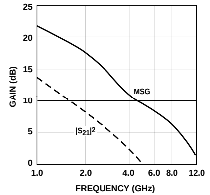
Figure 3. Insertion Power Gain, Maximum Available Gain and Maximum Stable Gain vs. Frequency. V_{DS} = 9\text{ V}, I_{DS} = 500\text{ mA} .
