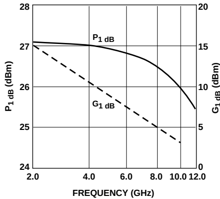
Figure 1. Power Output @ 1 dB Gain Compression and 1 dB Compressed Gain vs. Frequency.
