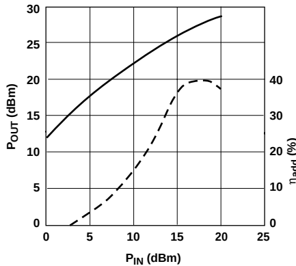
Figure 2. Output Power and Power Added Efficiency vs. Input Power.
