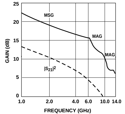
Figure 3. Insertion Power Gain, Maximum Available Gain and Maximum Stable Gain vs. Frequency.
