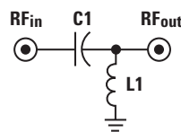
Figure 3. High Pass Circuit Topology.
