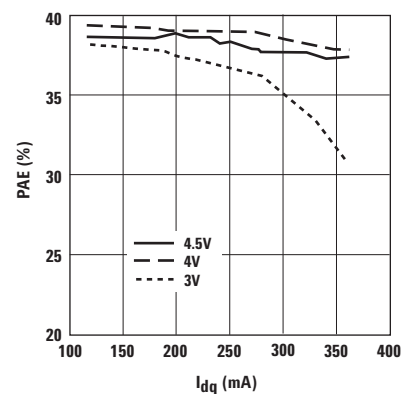
Figure 35. PAE @ P1dB vs. I_{dq} and V_{ds} at 3.9 GHz.
