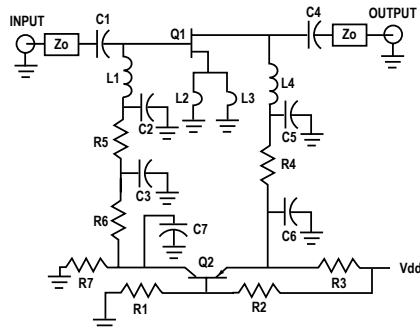
Figure 38. Typical ATF-551M4 LNA with Active Biasing.
