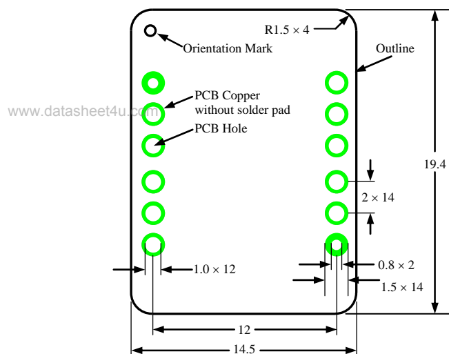
Figure 6 Top Side PCB Foot-print for the DIP Package
