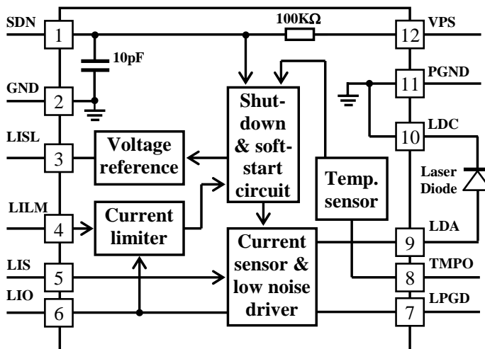
Figure 2 Block Diagram
