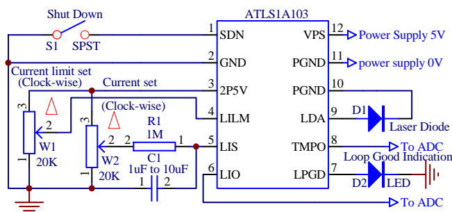
Figure 3 A Typical Stand-alone Application Schematic
