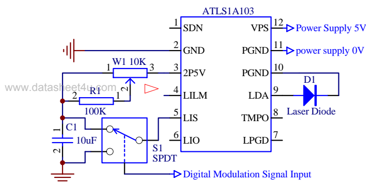
Figure 4 Low Noise Digital Modulation Circuit
