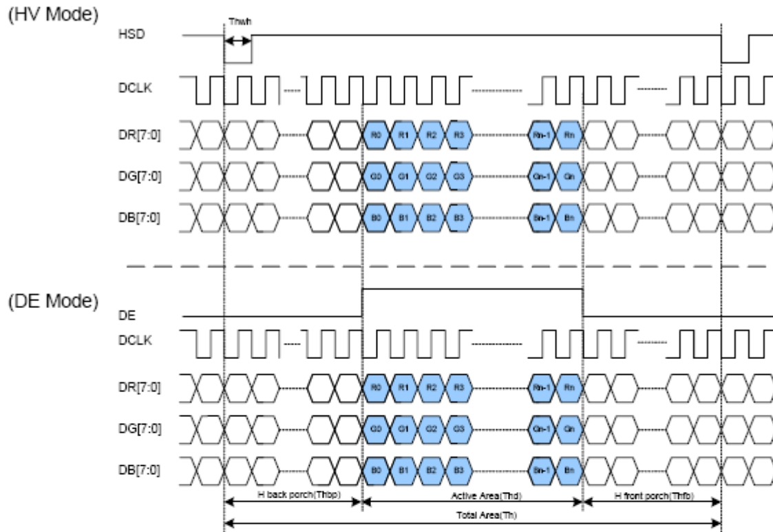
Parallel RGB input timing table
