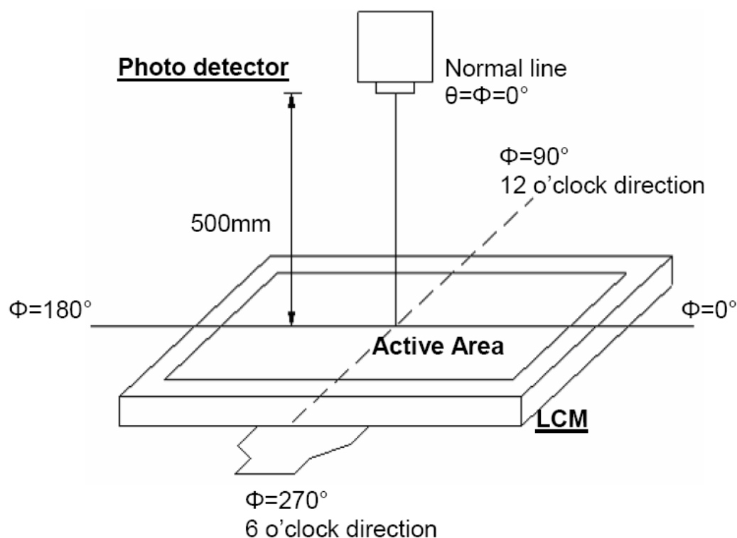
Figure 6.2 Optical measurement system setup
