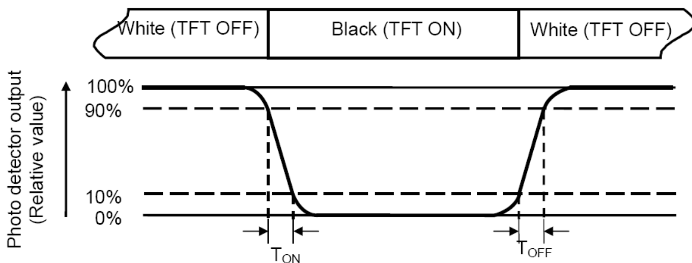
Figure 6.3 Definition of response.
