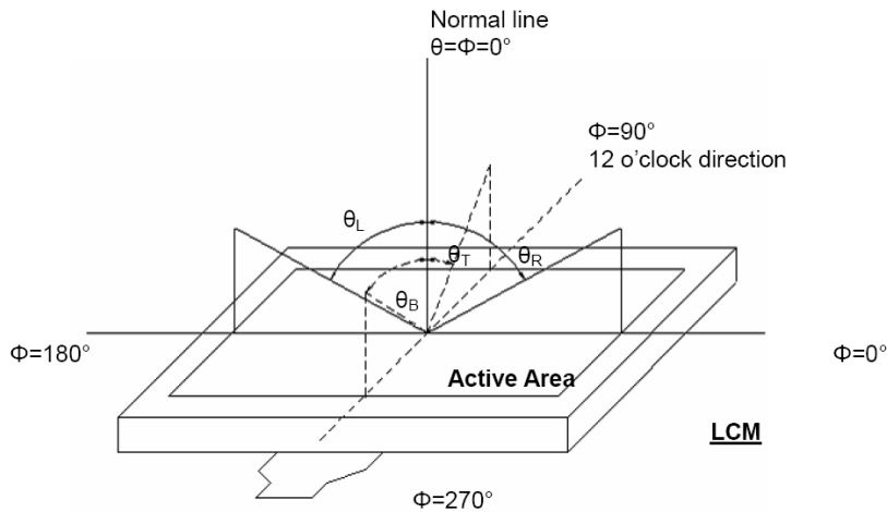
Figure 6.1 Definition of viewing angle.
