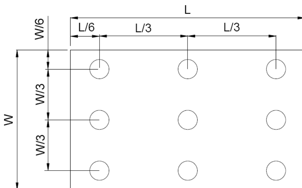
Figure 6.4 Definition of measuring points.
