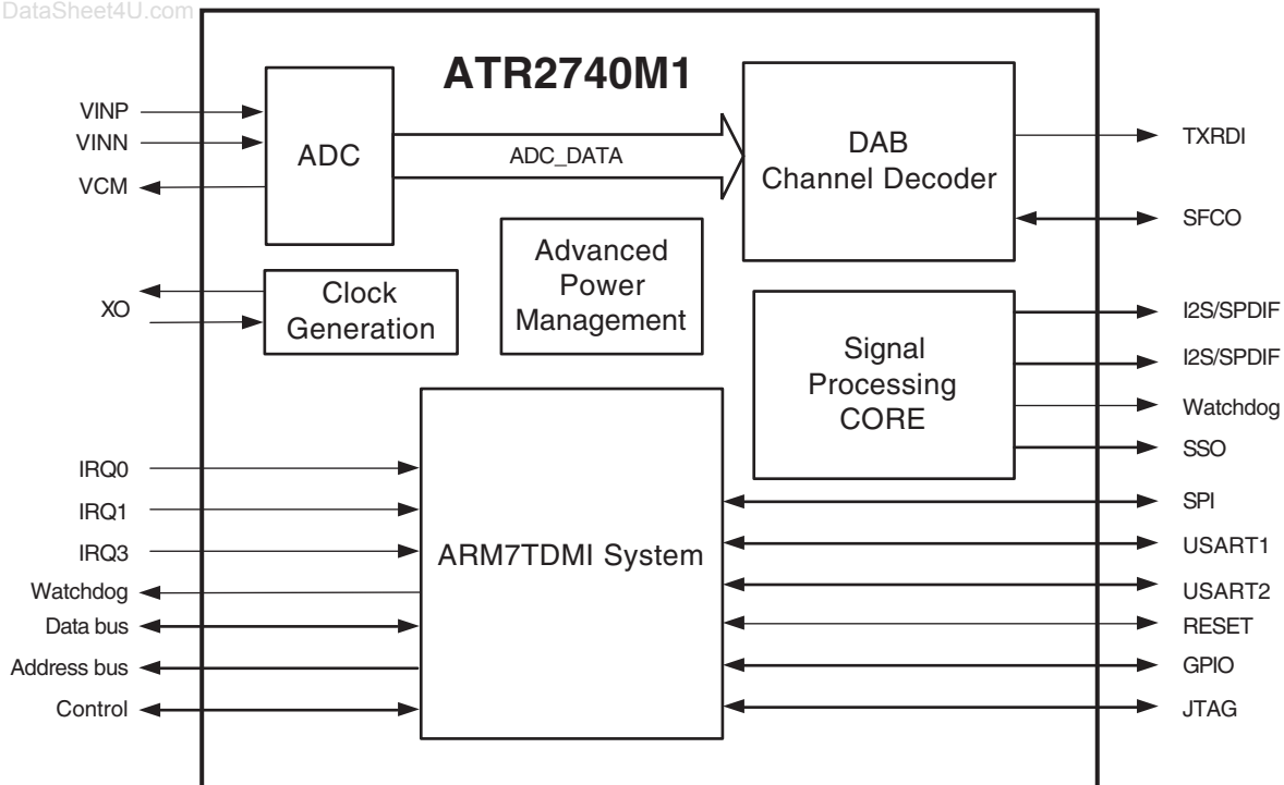
Figure 1-1. Block Diagram
