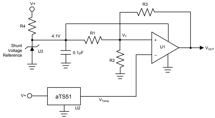
Figure 6. Thermostat/Fan Controller
