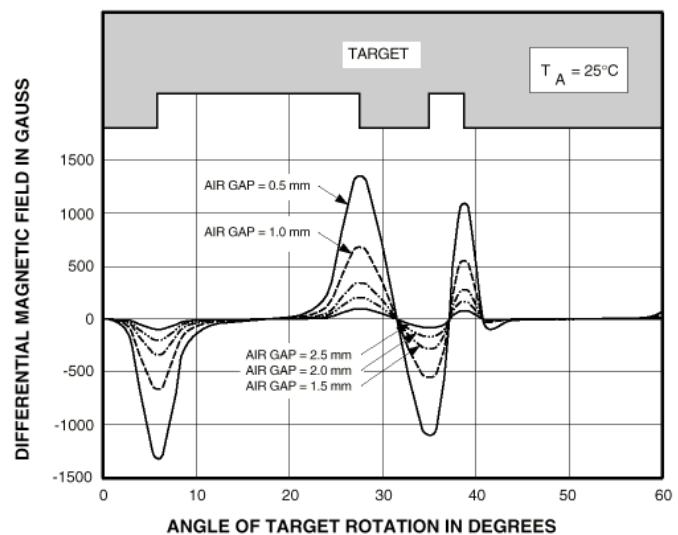
Figure 5. Affect of varying air gaps on differential sensors.
