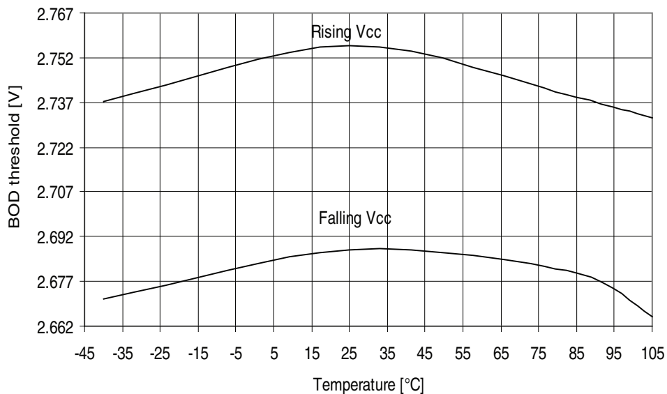
Figure 31-344. ATmega3250PA: BOD Thresholds vs. Temperature (BOD Level is 2.7V)
