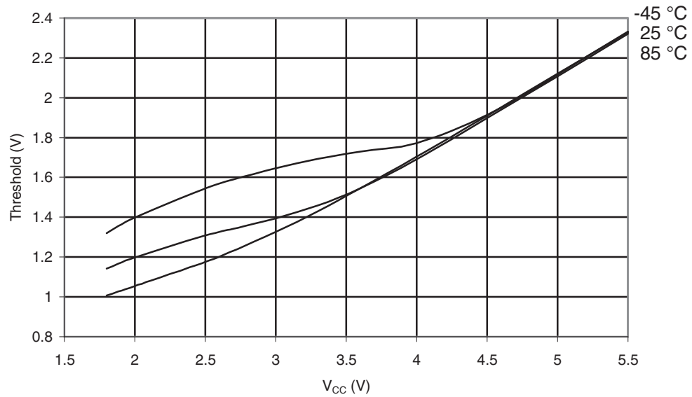
Figure 30-402. ATmega645A: Reset Input Threshold Voltage vs. V_{CC} ( V_{IH,Reset} , Reset Pin Read as "1")
