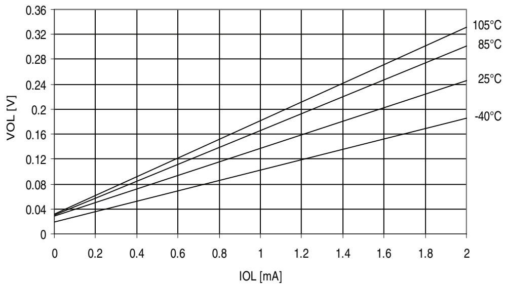
Figure 31-333. ATmega3250PA: I/O Pin Output Voltage vs. Sink Current, Ports A, C, D, E, F, G ( V_{CC} = 1.8V )
