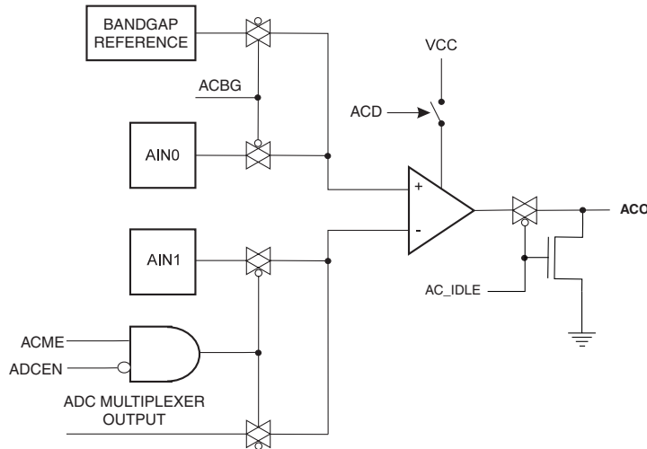
Figure 113. Analog Comparator
