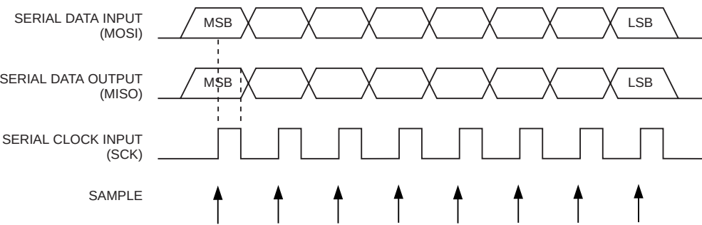
Figure 129. Serial Programming Waveforms
