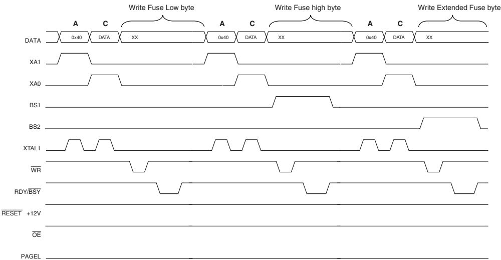
Figure 123. Programming the FUSES Waveforms
