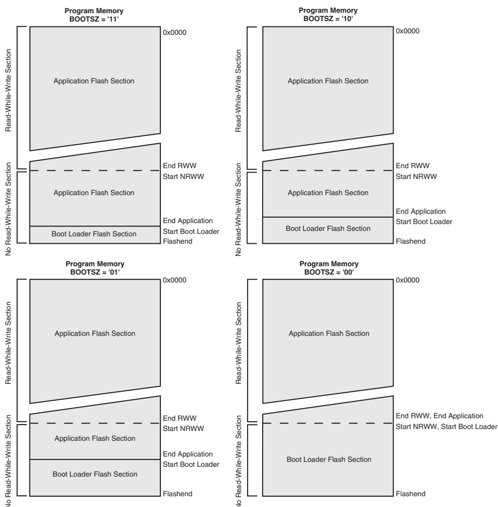
Figure 117. Memory Sections
