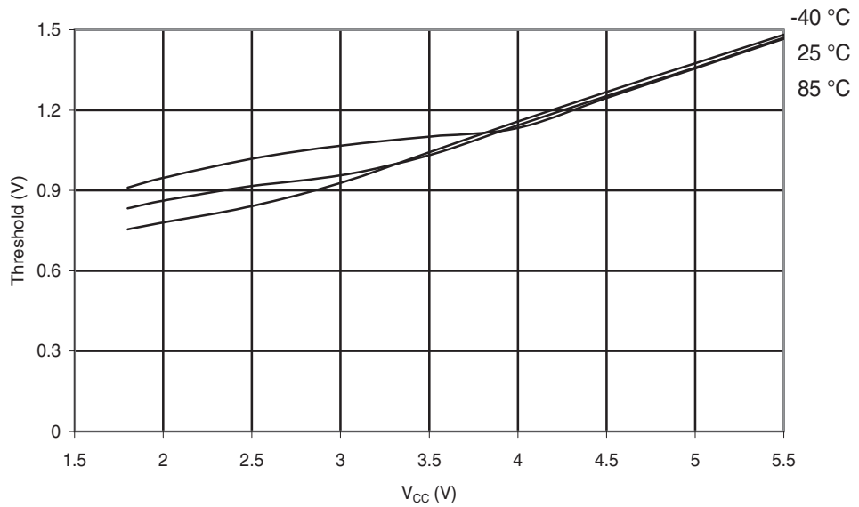
Figure 31-122. ATmega88A: Reset Input Threshold Voltage vs. V_{CC} ( V_{Ith} I/O Pin read as '1')
