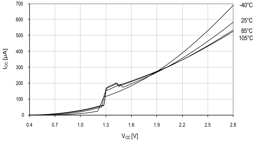
Figure 34-143. Power-on Reset Current Consumption vs. V_{CC} BOD level = 3.0V, enabled in sampled mode
