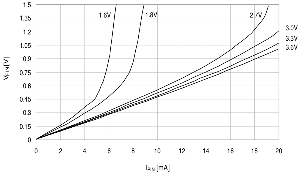
Figure 34-110. I/O Pin Output Voltage vs. Sink Current
