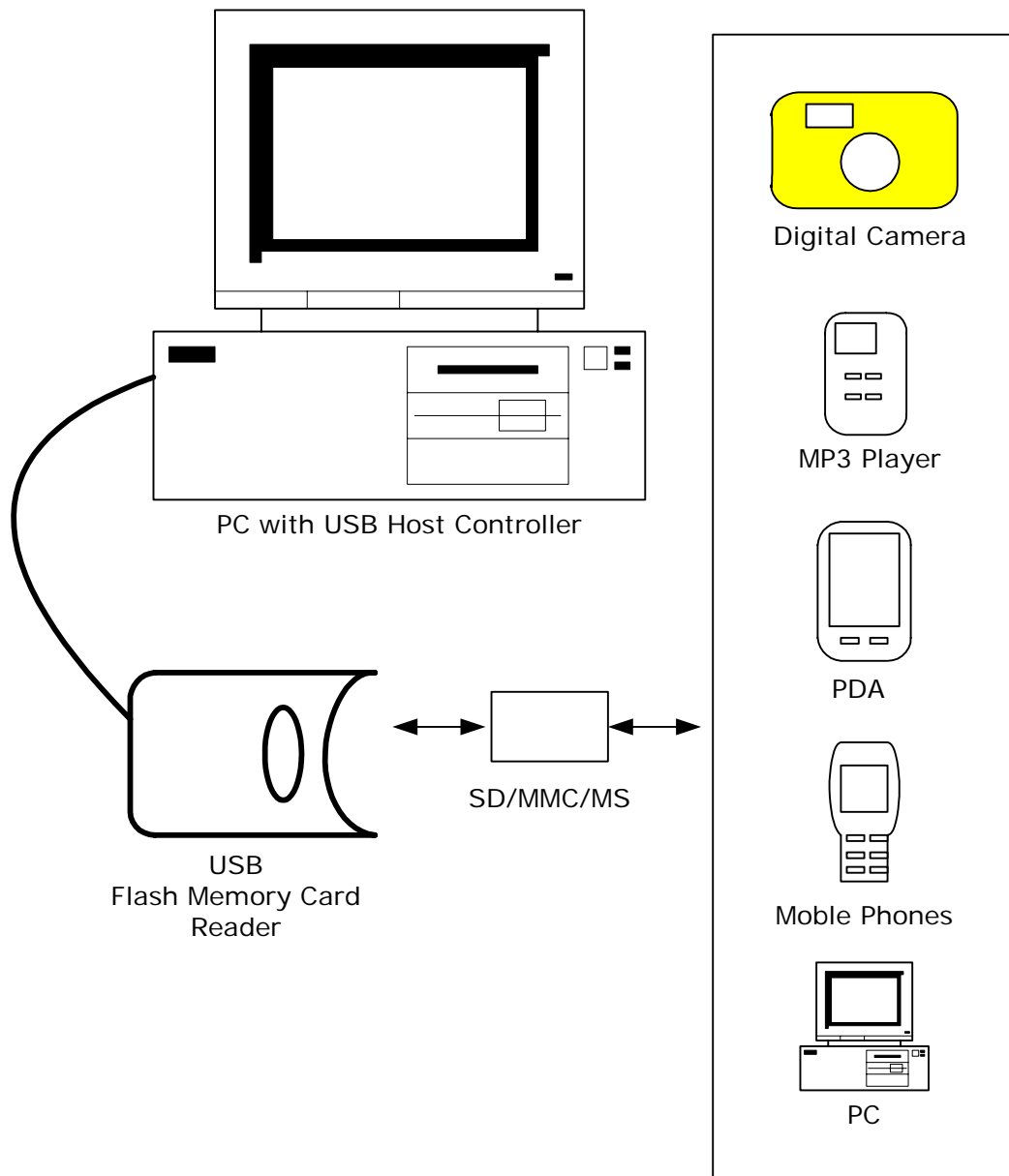
Figure 2.1 Block Diagram
