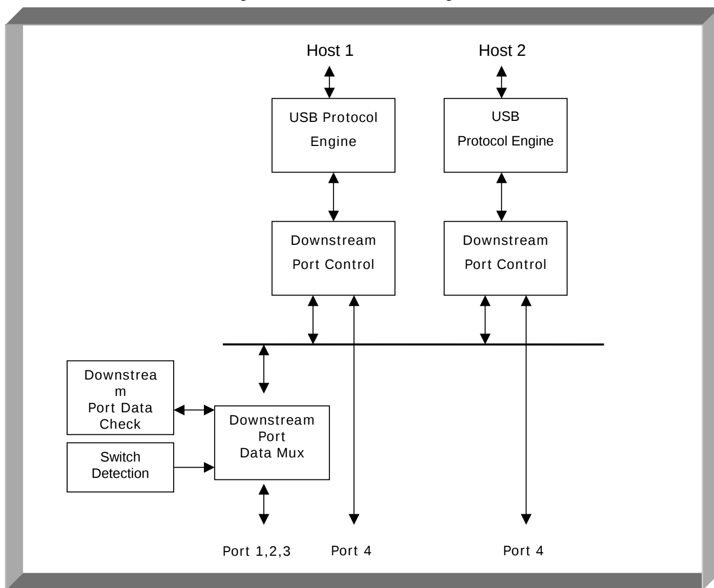
Figure 4.1 AU9223 Block Diagram
