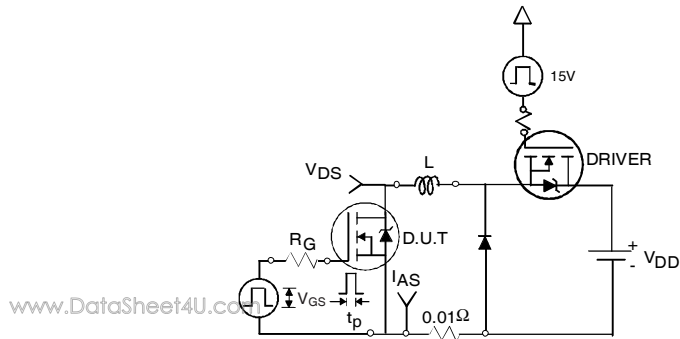
Fig 12a. Unclamped Inductive Test Circuit
