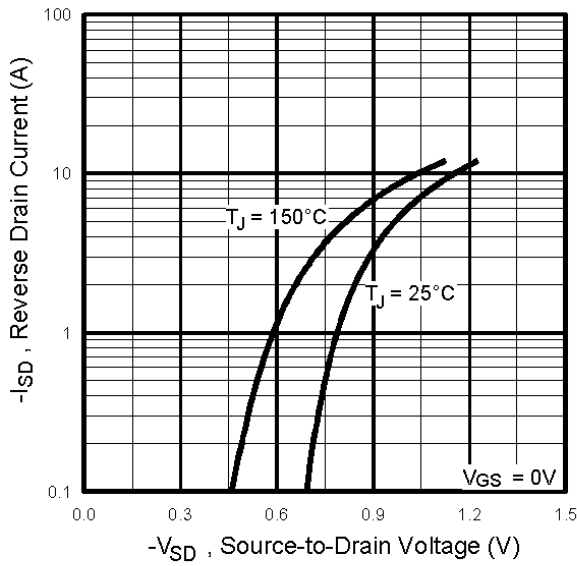
Fig 18. Typical Source-Drain Diode Forward Voltage
