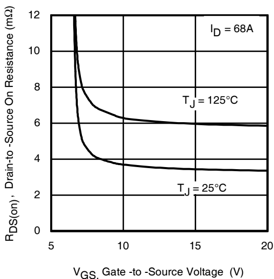
Fig 3. Typical On-Resistance vs. Gate Voltage
