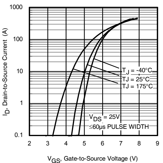
Fig 5. Transfer Characteristics
