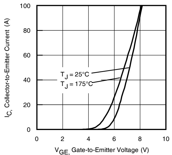
Fig. 9 - Typ. Transfer Characteristics V_{CE} = 50\text{V} ; t_p = 30\mu\text{s}
