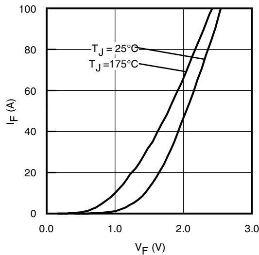
Fig. 12 - Typ. Diode Forward Characteristics t_p = 30\mu s
