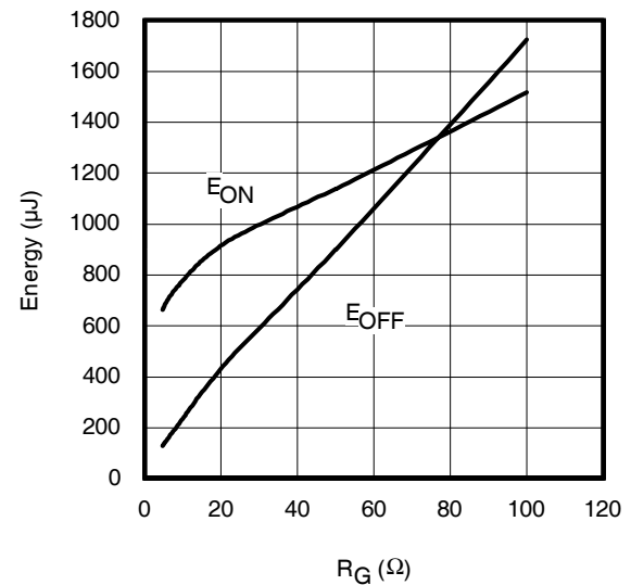
Fig. 15 - Typ. Energy Loss vs. R_G T_J = 175^\circ C ; L = 0.49mH ; V_{CE} = 400V ; I_{CE} = 20A ; V_{GE} = 15V
