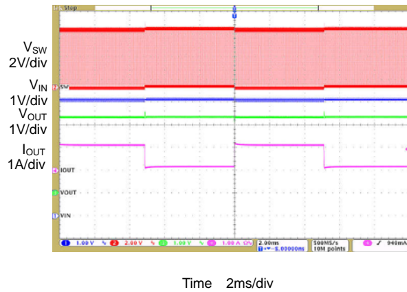
Figure 24. Dynamic Mode ( I_{LOAD}=200\text{mA} to 1200\text{mA} , V_{IN}=5\text{V} , V_{OUT}=3.3\text{V} )
