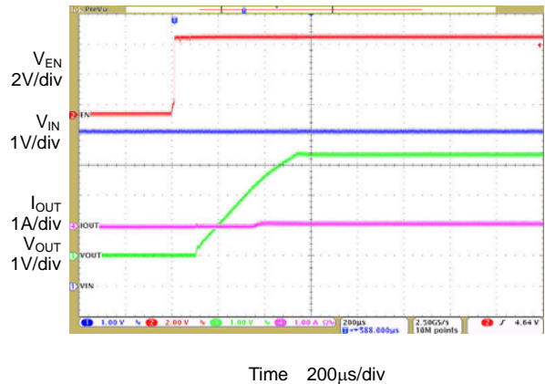
Figure 27. EN Pin L to H ( V_{IN}=5\text{V} , V_{OUT}=3.3\text{V} , I_{OUT}=100\text{mA} )
