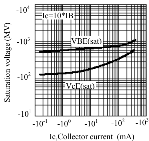
Fig.4 Saturation voltage
