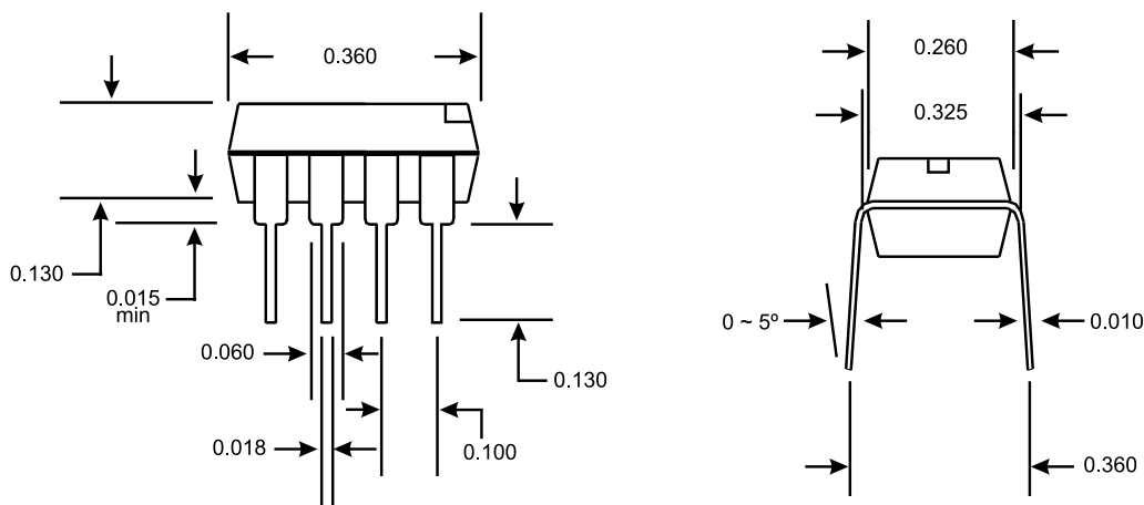
8 - Pin DIP
