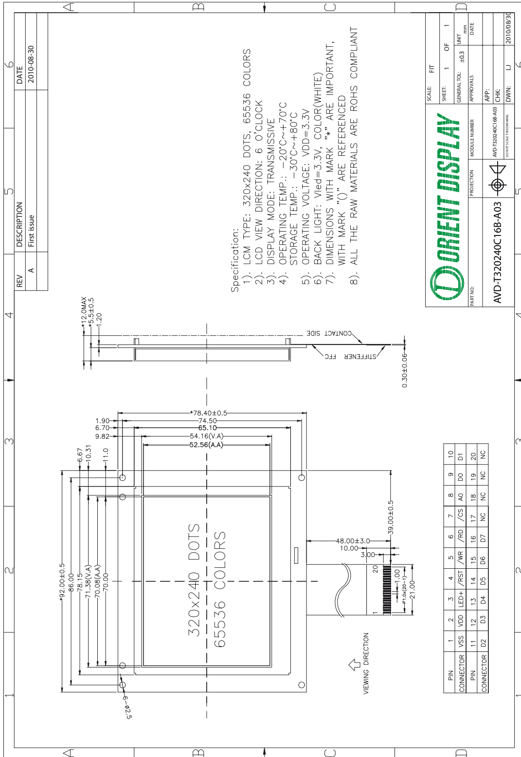
Figure 2 Dimensional outline
